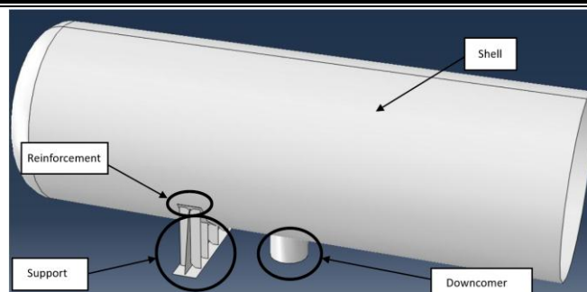
Fig. 3 3D-shell model used for finite element analysis
