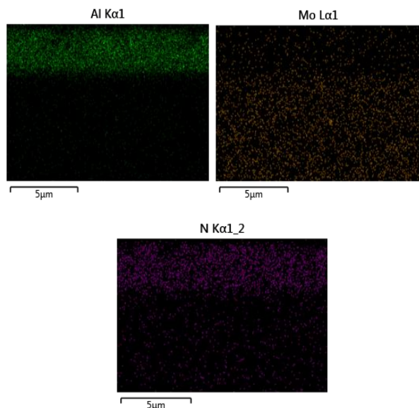
Fig. 10 EDX surface elemental analysis of the nACRo 4 coating
