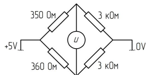
Fig. 3 Bridge circuit.
