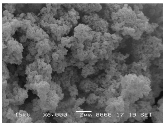
Fig. 4a Microscopic image of synthesized polyaniline salts H 3 PO 4
