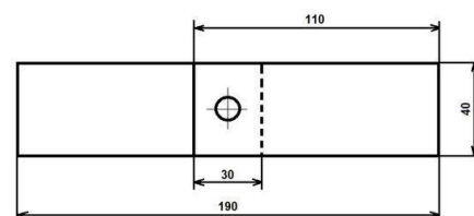
Figure 1: Shape and dimensions of test specimens and joints designed for FD long \varnothing 5.3 mm tool
